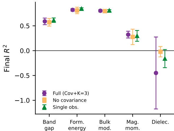
(b) Residual-coupled variant ablation
