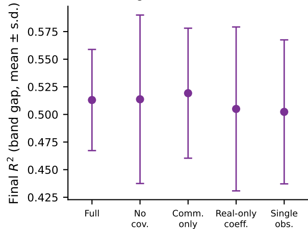
(a) Original formalism ablation
