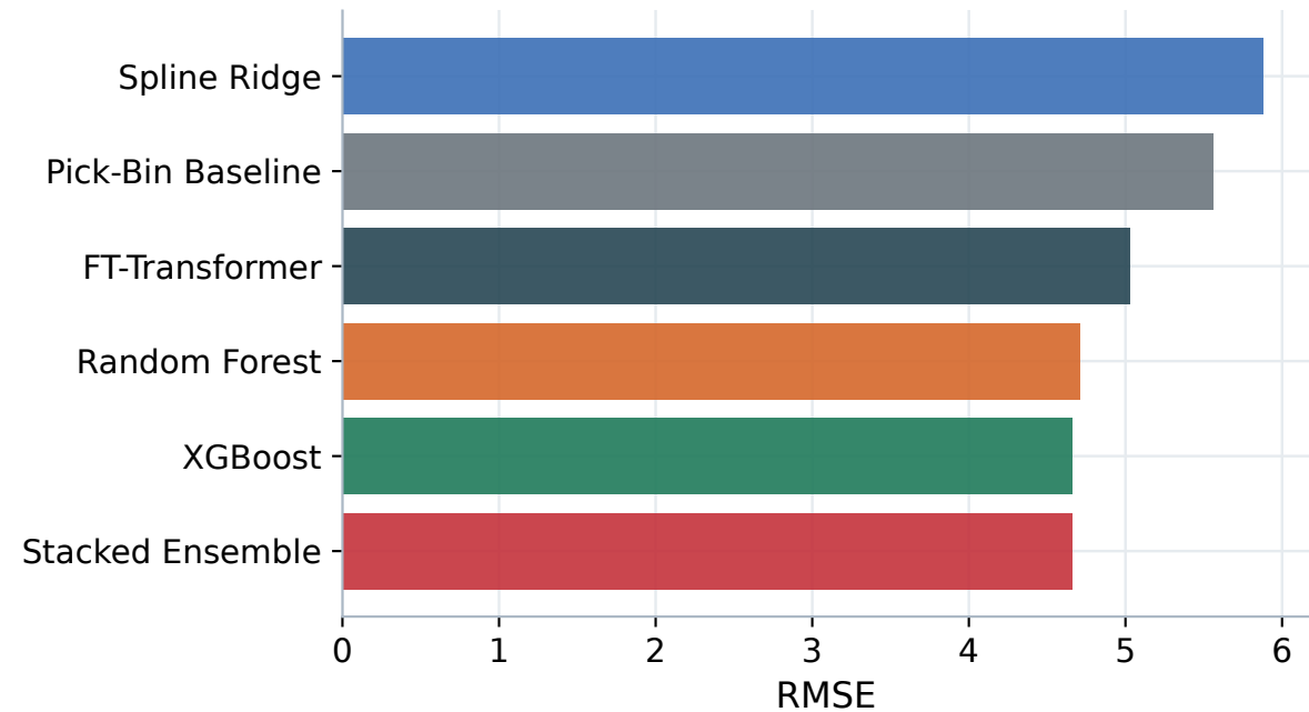
RMSE
