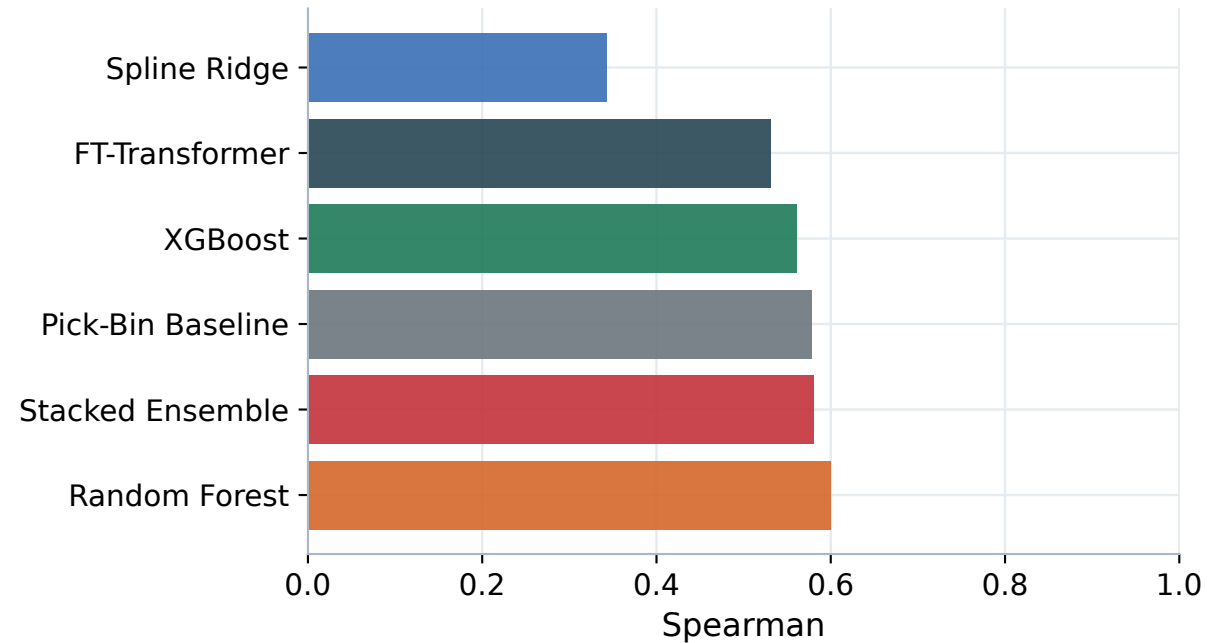
Spearman
