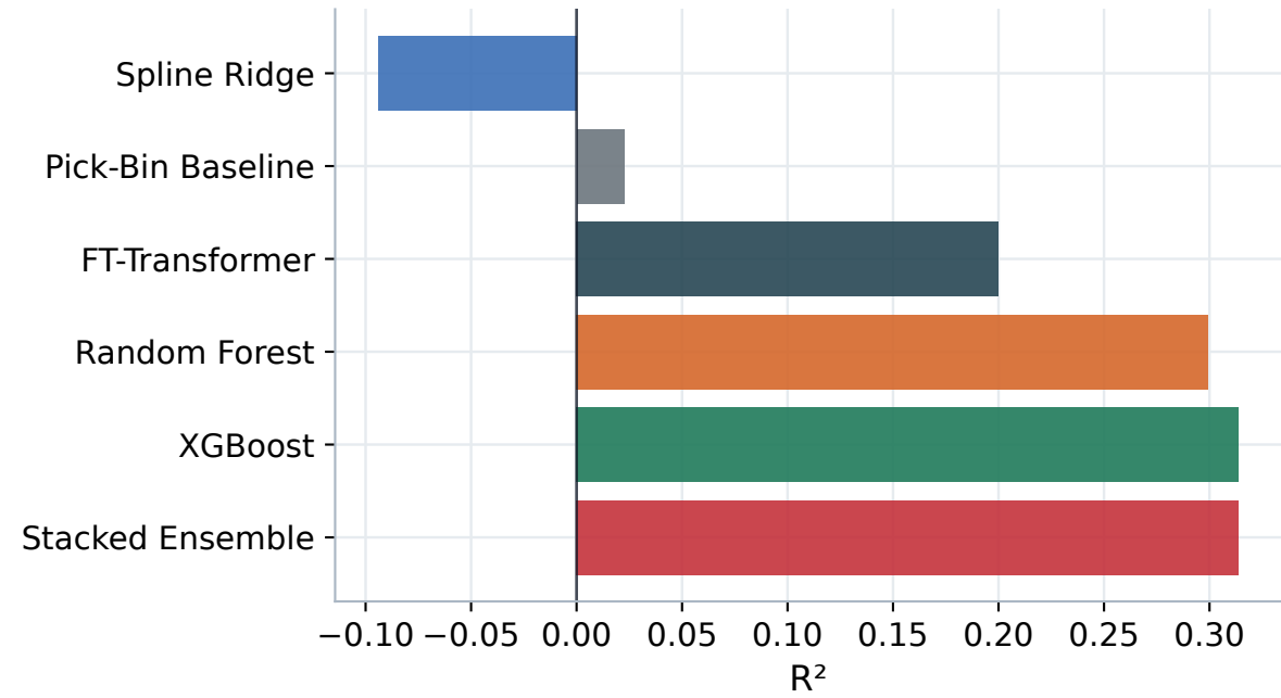
R 2
