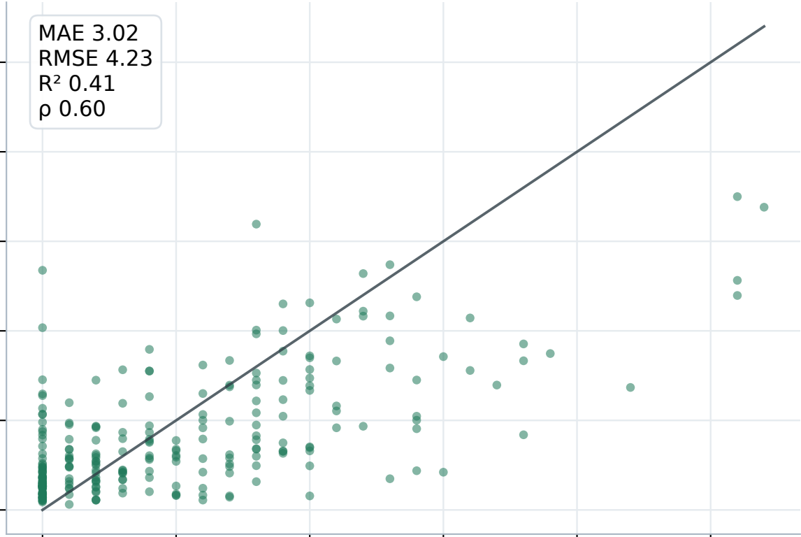
FT-Transformer
