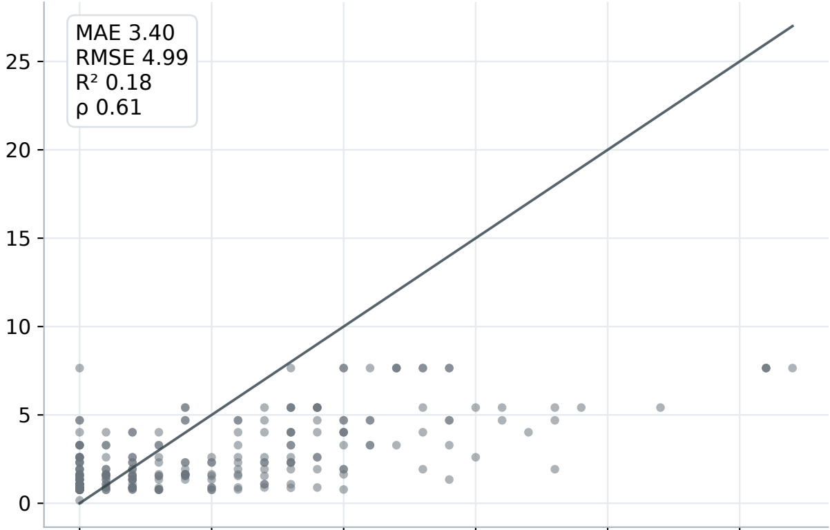
Random Forest
