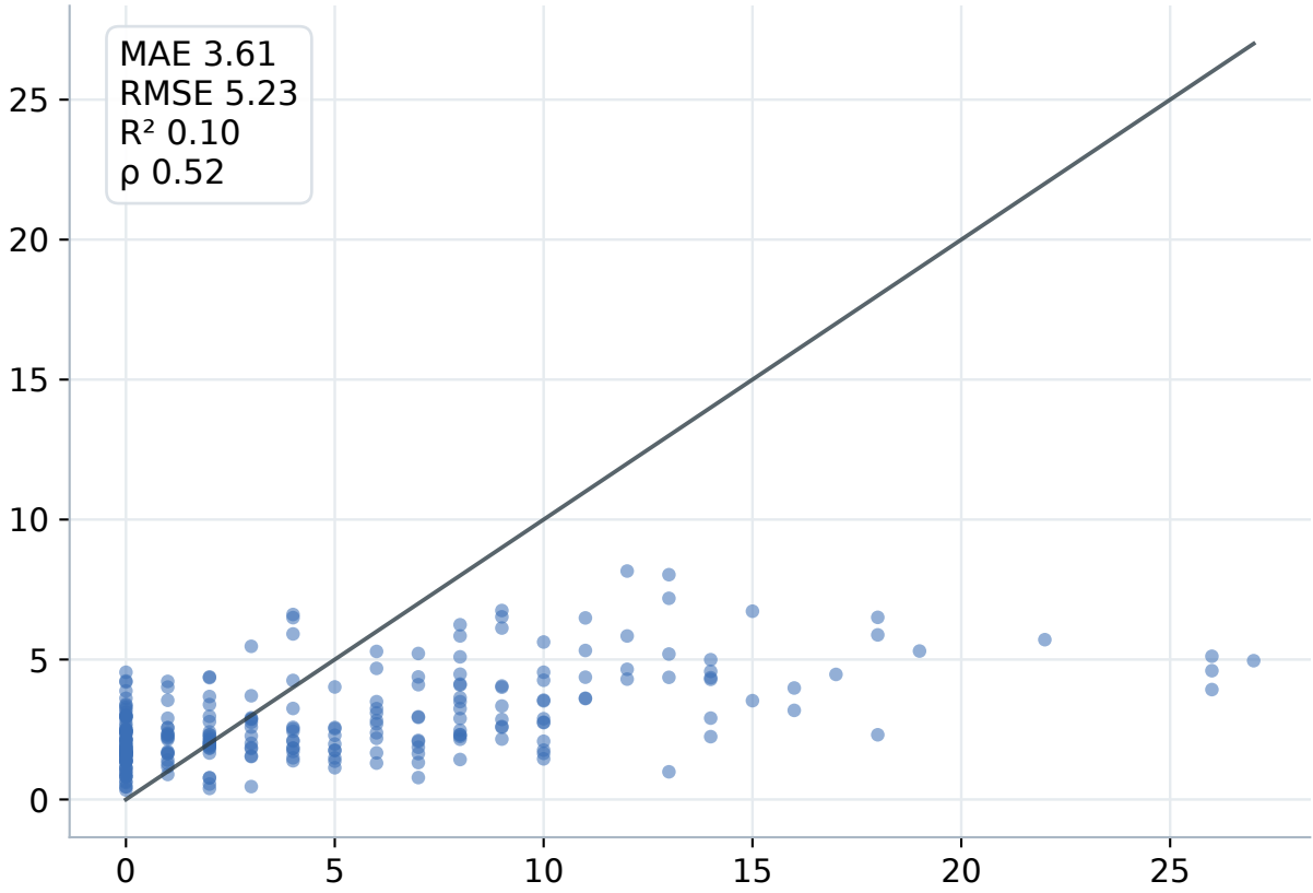
Spline Ridge
