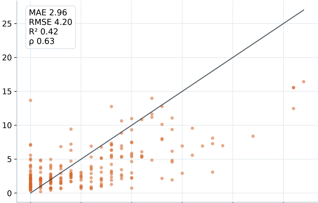
Spline Ridge
