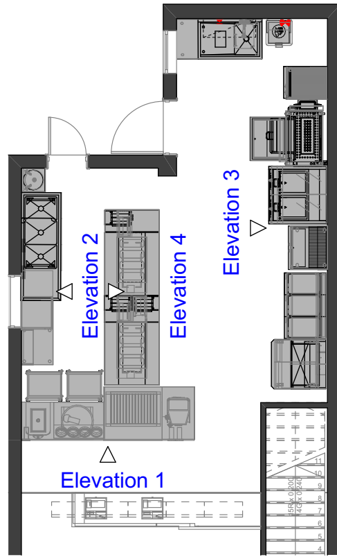
0. Elevations plan 1:100
