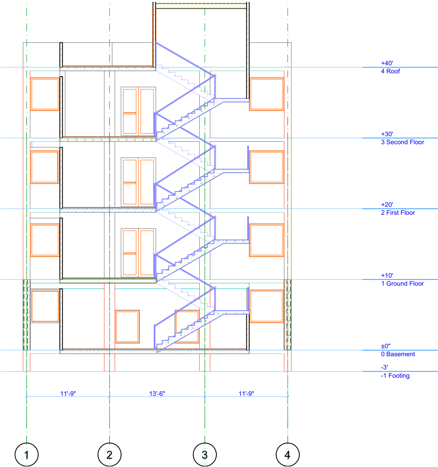
Building Section
