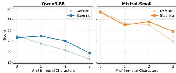
Figure 4: Comparison of steering performance and mitigation results across models. Y-axis of the lower figure indicates the CoSER score.
