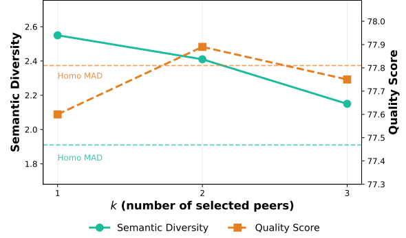
Figure 6: Sensitivity of Creative-MAD to the peer selection hyperparameter k on Qwen3-8B.
