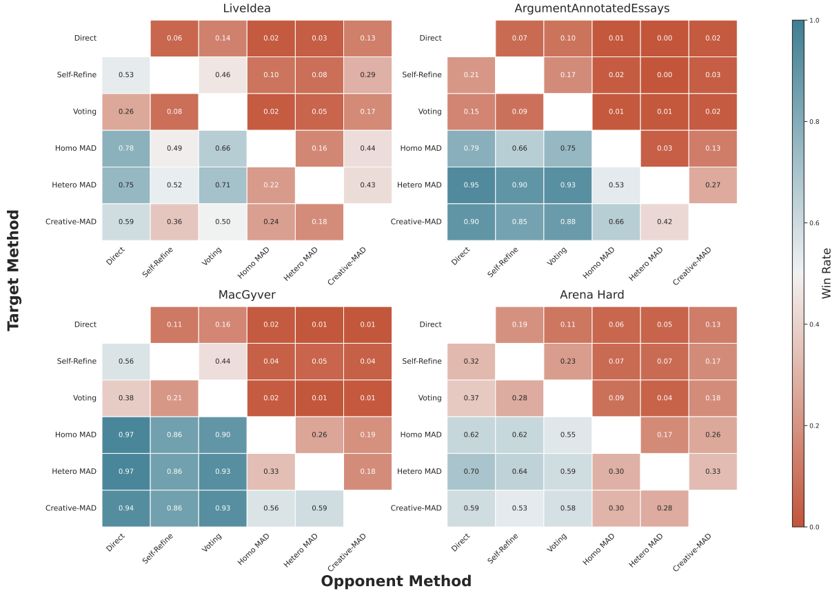
Figure 7: Pairwise win rate heatmaps across four benchmarks on Qwen3-8B. Each cell (i, j) denotes the win rate of the target method (row) against the opponent method (column).
