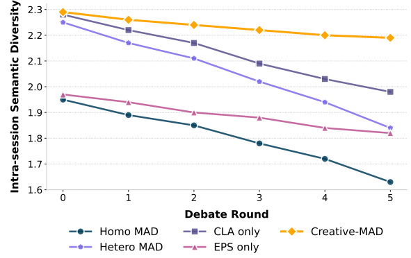
Figure 3: Intra-session semantic diversity across debate rounds for each method variant on Qwen3-8B, averaged across four benchmarks.
