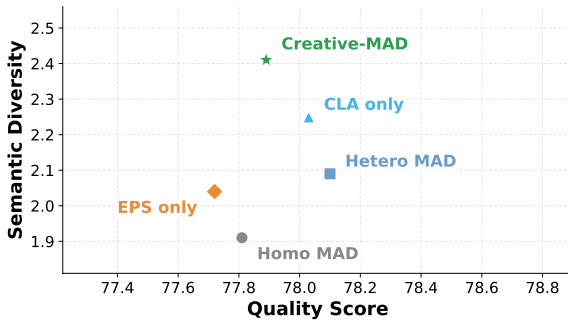
Figure 5: Semantic diversity versus quality score for Creative-MAD ablation variants and baselines on Qwen3-8B, averaged across four benchmarks.
