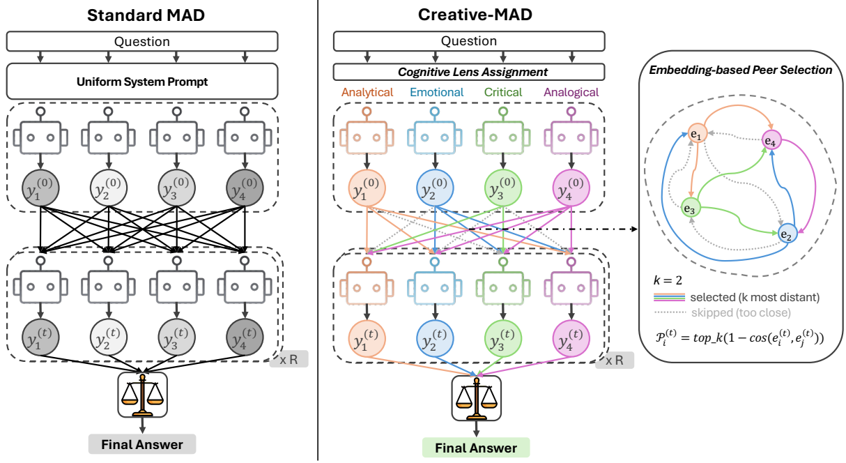
Figure 1: Comparison of Standard MAD and Creative-MAD. Standard MAD’s uniform prompts and full peer connectivity drive convergence across debate rounds. Creative-MAD addresses this via Cognitive Lens Assignment (CLA), anchoring each agent to a distinct cognitive mode, and Embedding-based Peer Selection (EPS), restricting each agent to its k most semantically distant peers.
