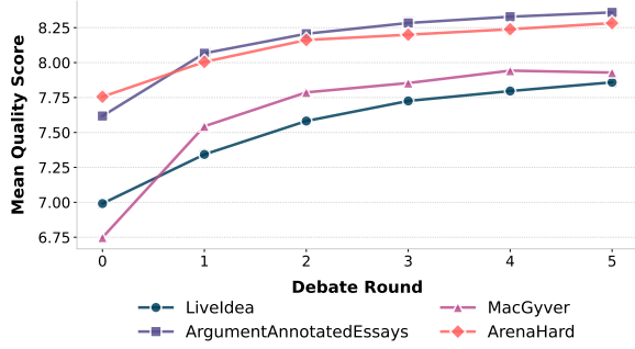
Figure 2: Mean quality score of Creative-MAD across debate rounds on Qwen3-8B.
