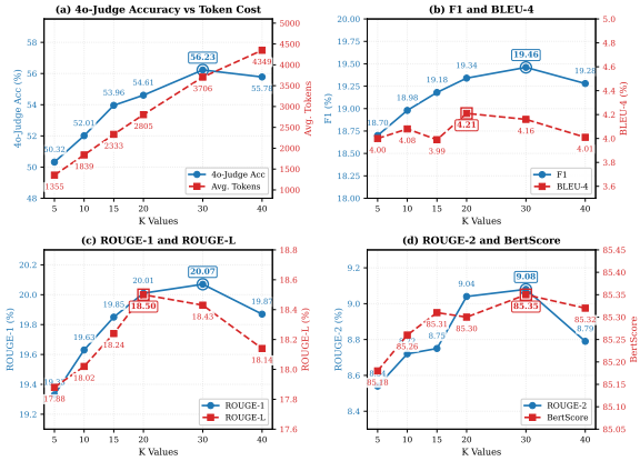
Figure 2: Sensitivity of retrieval budget k on LoCoMo. (a) 4o-Judge accuracy and token cost. (b) F1, BLEU-4. (c) ROUGE-1/L. (d) ROUGE-2, BertScore.
