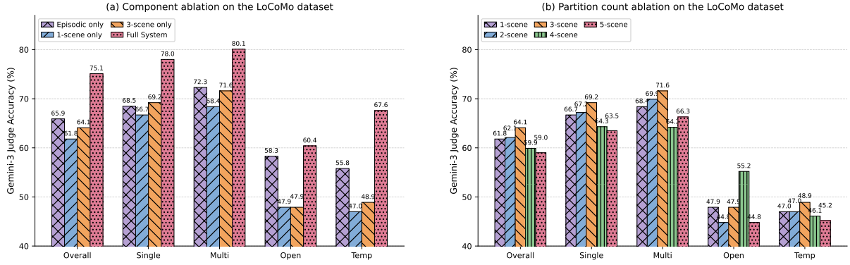
Figure 3: Ablation results on the LoCoMo dataset. (a) Component ablation. (b) Partition count ablation.
