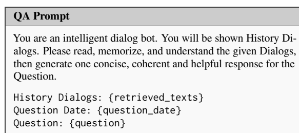
Figure 9: QA prompt used to generate responses, identical to that of MemGAS (Xu et al., 2026) (following Lu et al., 2023; Pan et al., 2025).
