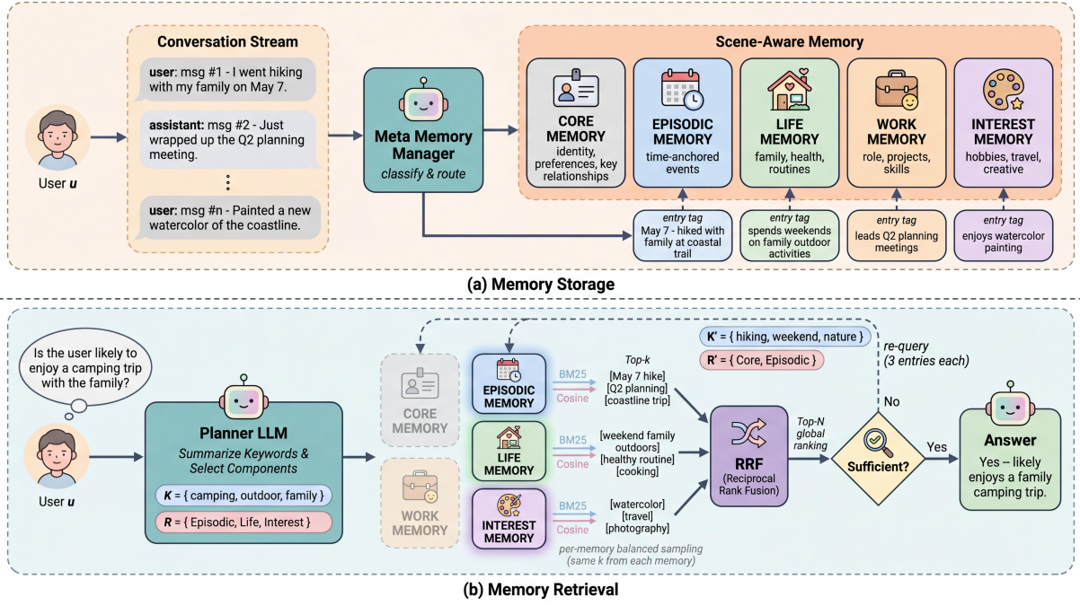
Figure 1: Overview of the CreaMem architecture, consisting of a Meta Memory Manager, an Episodic Memory, three Life Scene Memories, and a Core Memory.
