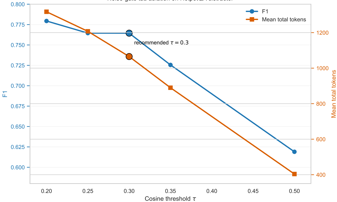
Noise-gate tau ablation on HotpotQA distractor
