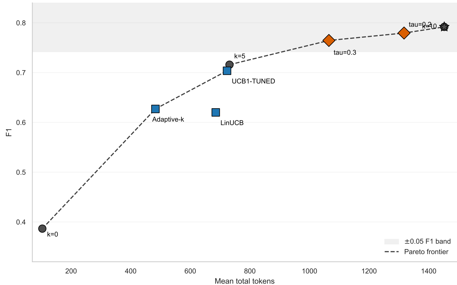
HotpotQA distractor: quality-cost frontier
