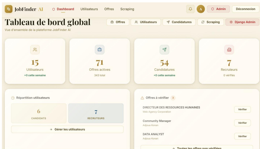
Figure 27 : Dashboard Admin
