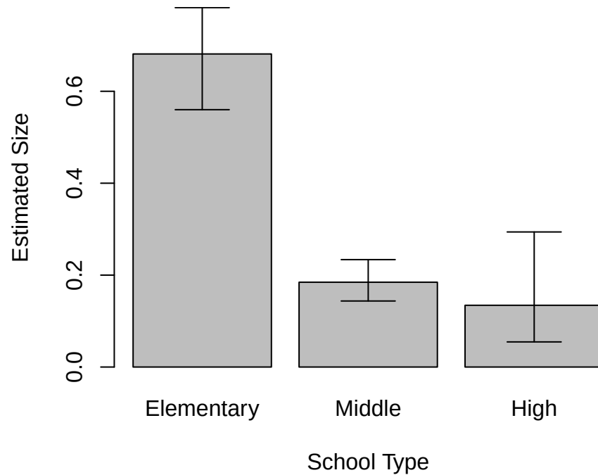
Figure 7.9: Estimated proportions of schools by school type - with asymmetric confidence intervals
