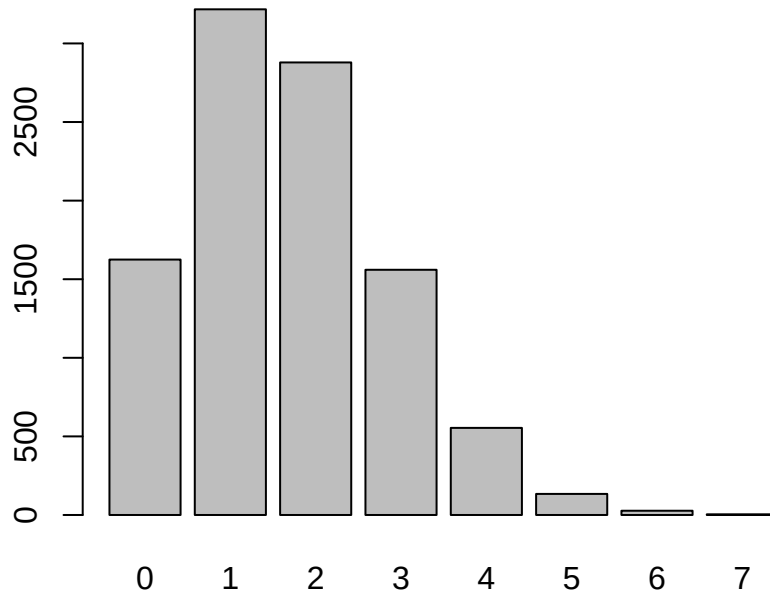
Figure 2.9: 10000 draws from a Binomial(10,1/6)
