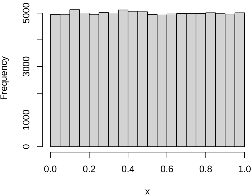
Histogram of runif(1e+05)
