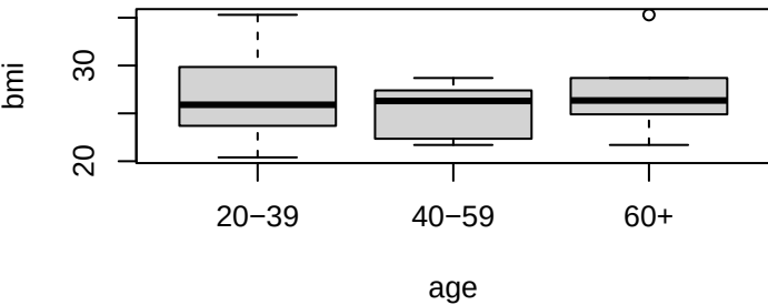
Hot deck imputation
