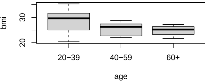
Original data set
