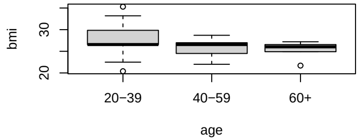
Cell mean imputation
