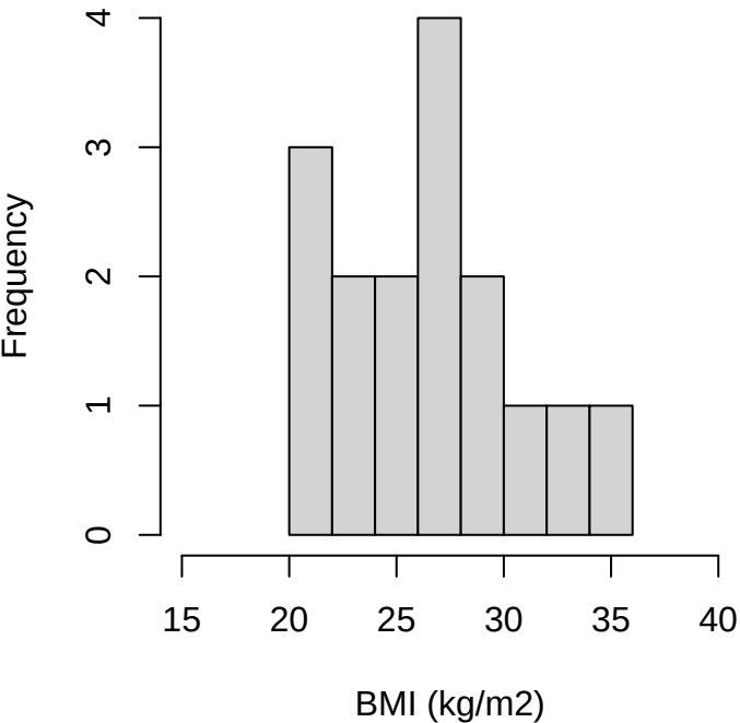
BMI distribution before imputation
