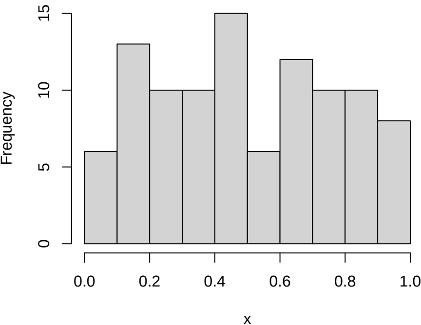
Histogram of runif(100)
