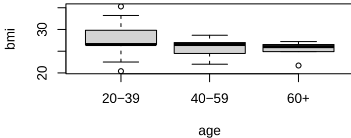
Mean imputation
