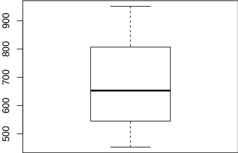
API (2000) Scores
