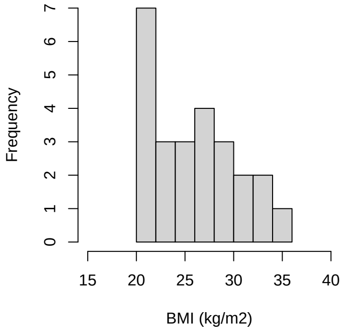
BMI distribution after imputation
