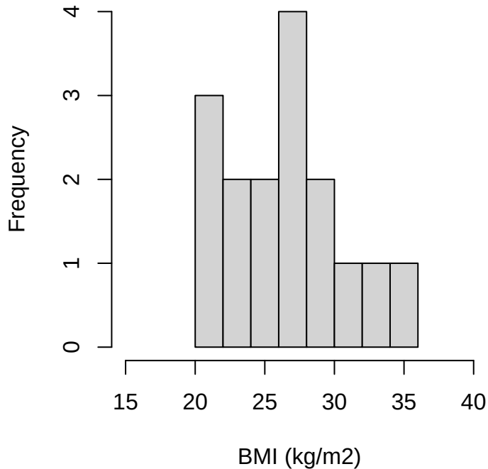
BMI distribution before imputation
