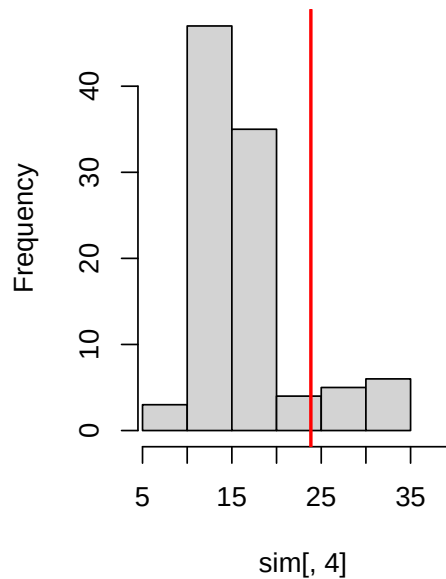
SE of Postratified estimates
