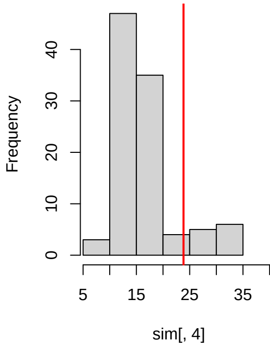
SE of Postratified estimates
