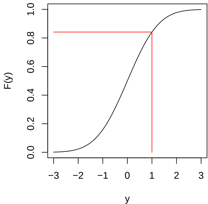
F(1)=\Pr(Y<1)=0.8413
