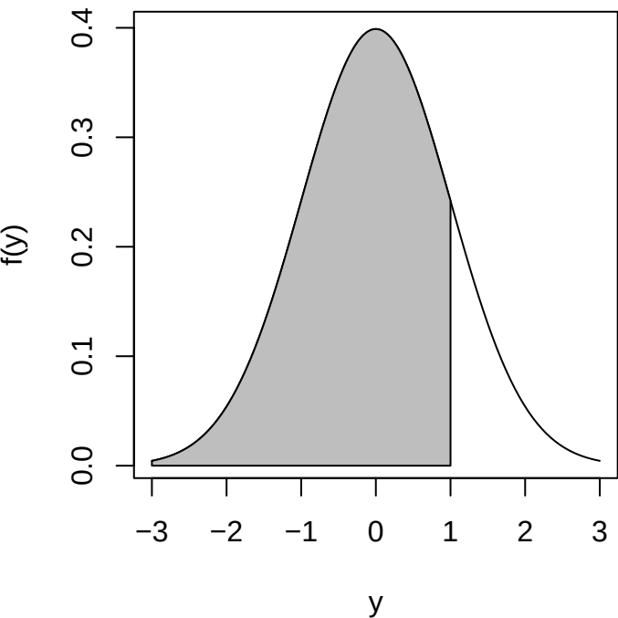
Normal density
