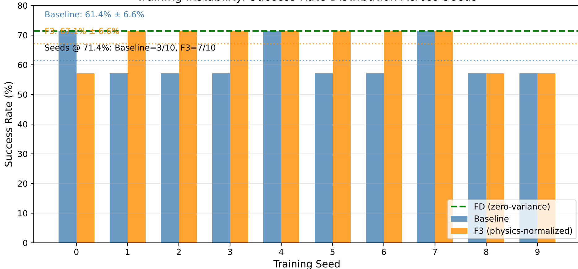
Training Instability: Success Rate Distribution Across Seeds
