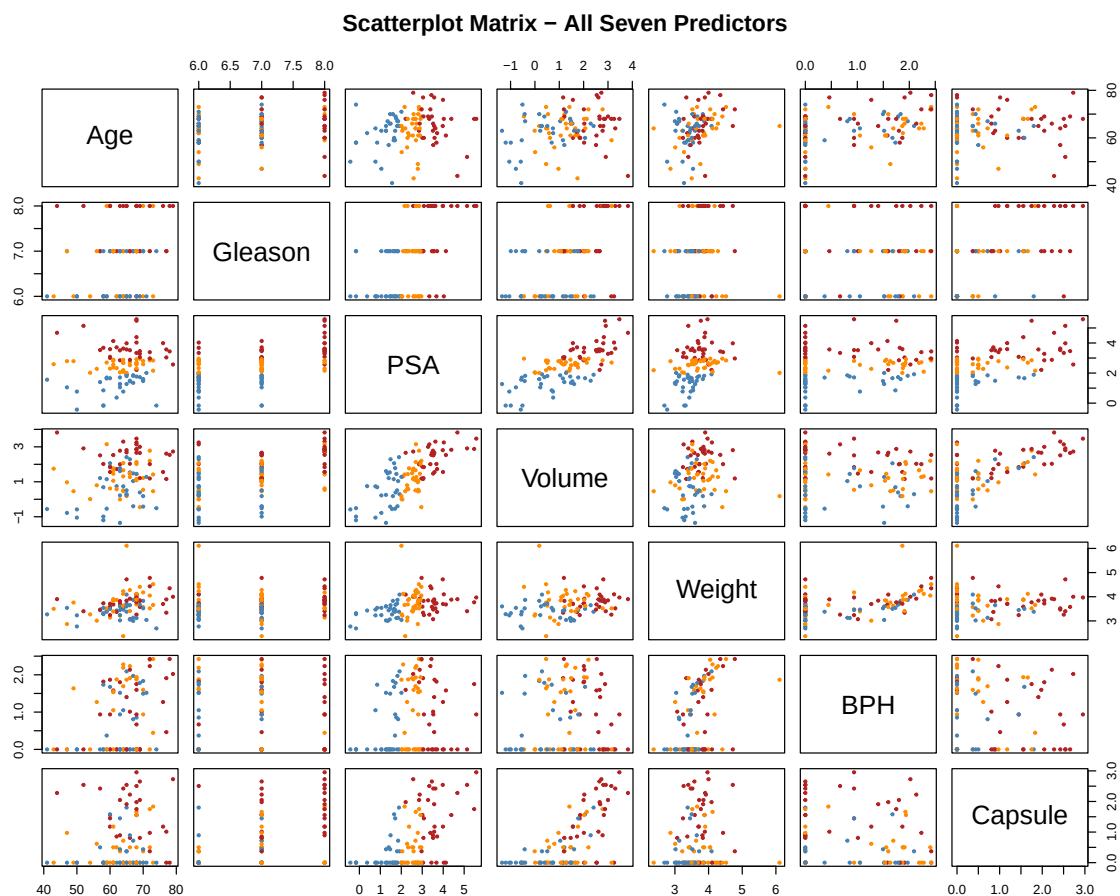
Figure 5: Scatterplot matrix of all seven transformed quantitative variables
