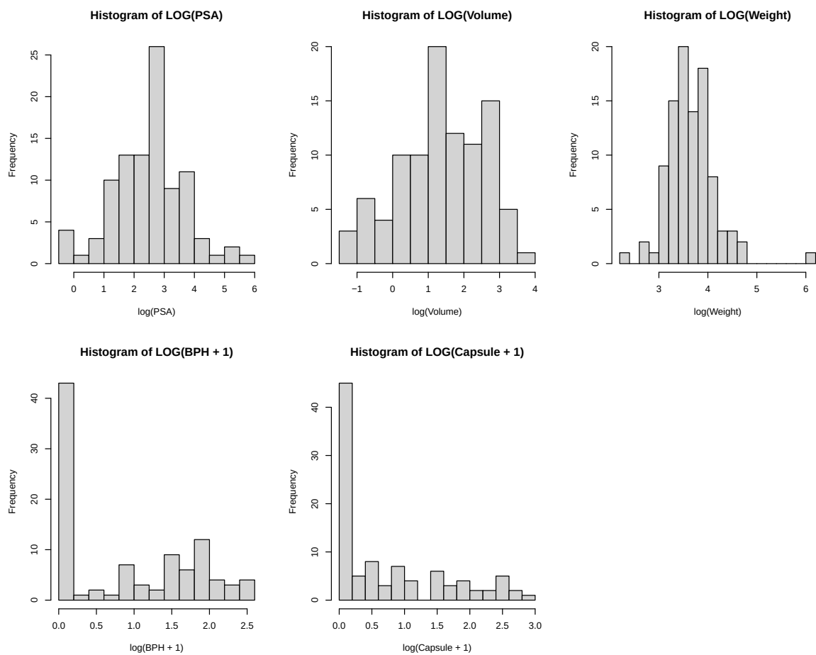
Figure 2: Histograms for all transformed variables
