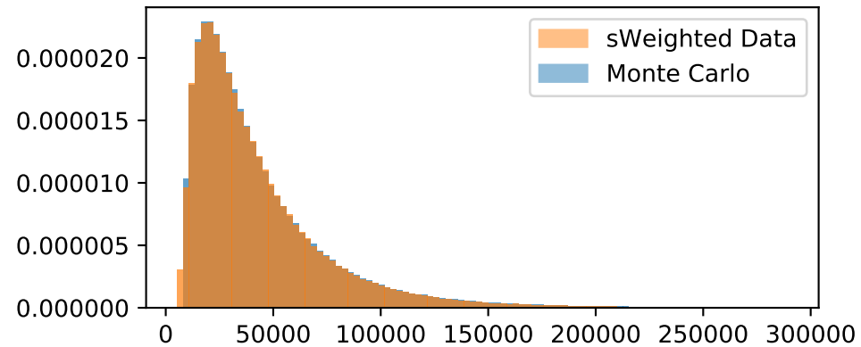
mu_P
