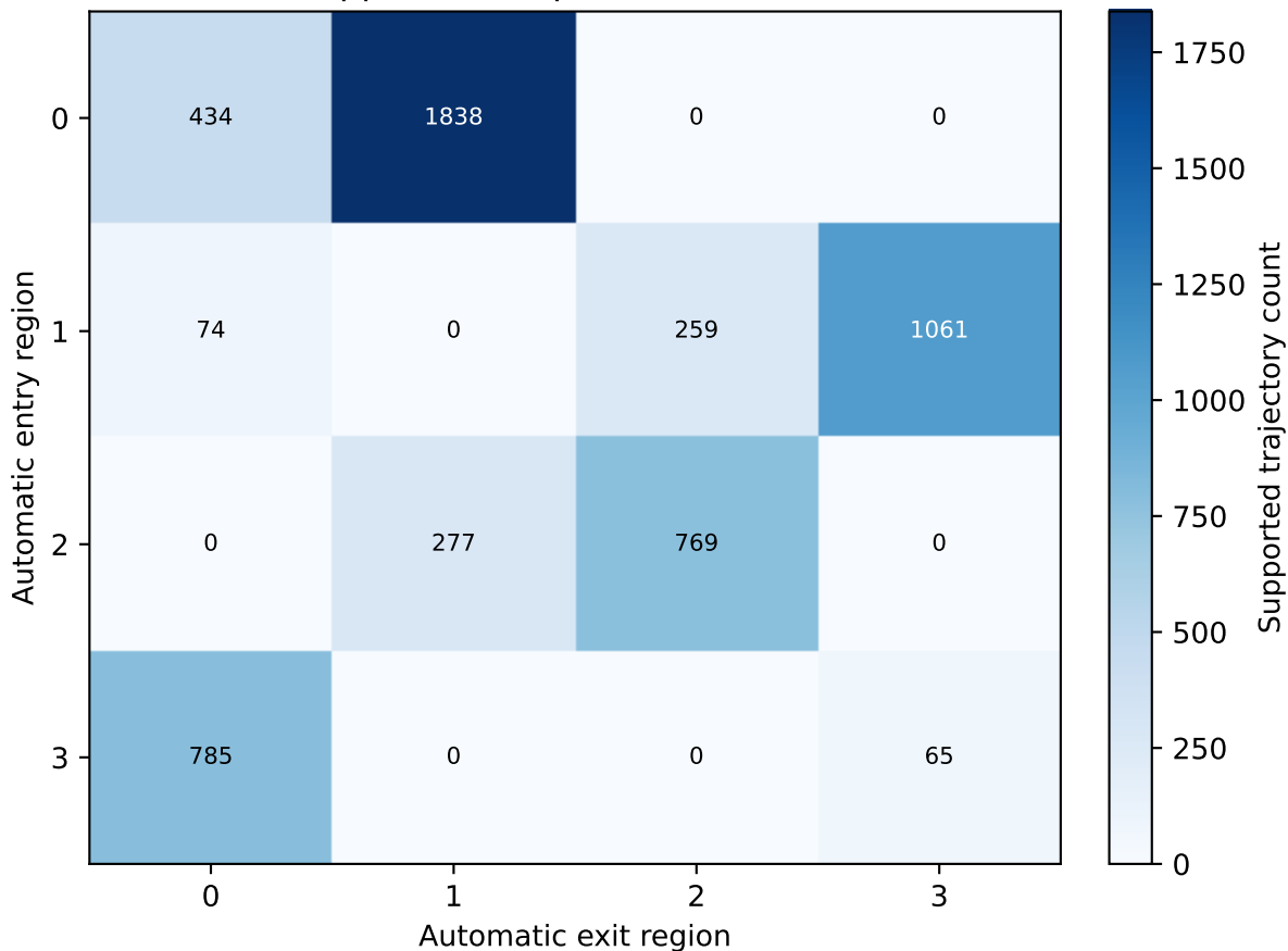
NE8th: supported OD pairs (threshold=0.50%)
