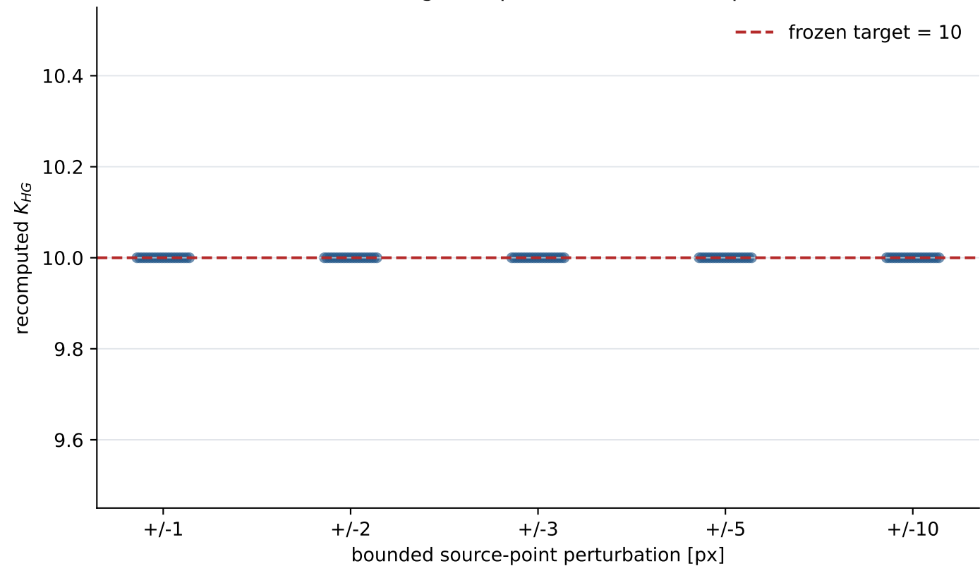
116th / NE12th: target response to calibration perturbation
