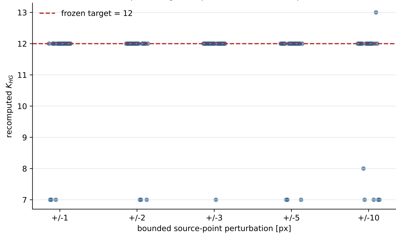
150th / Newport: target response to calibration perturbation
