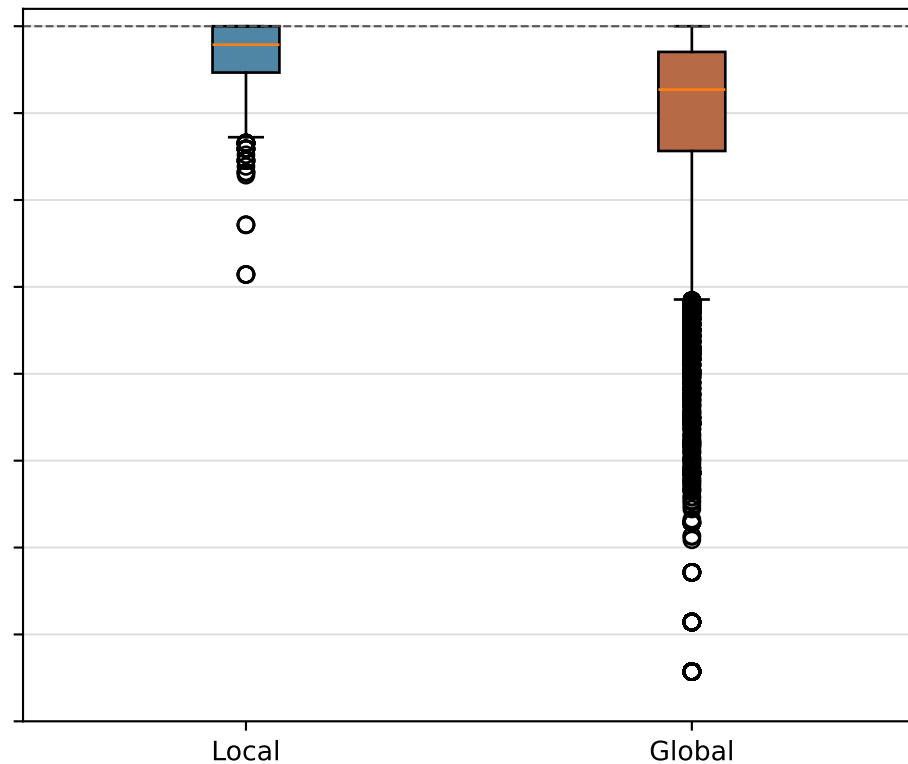
Kendall rank correlation
