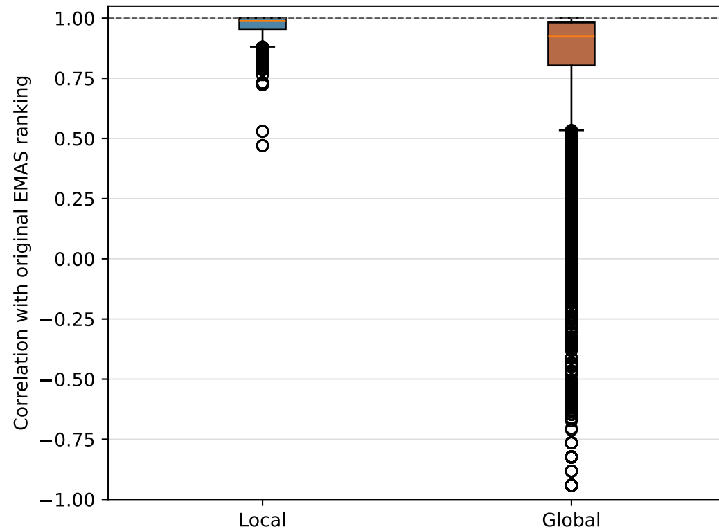
Spearman rank correlation
