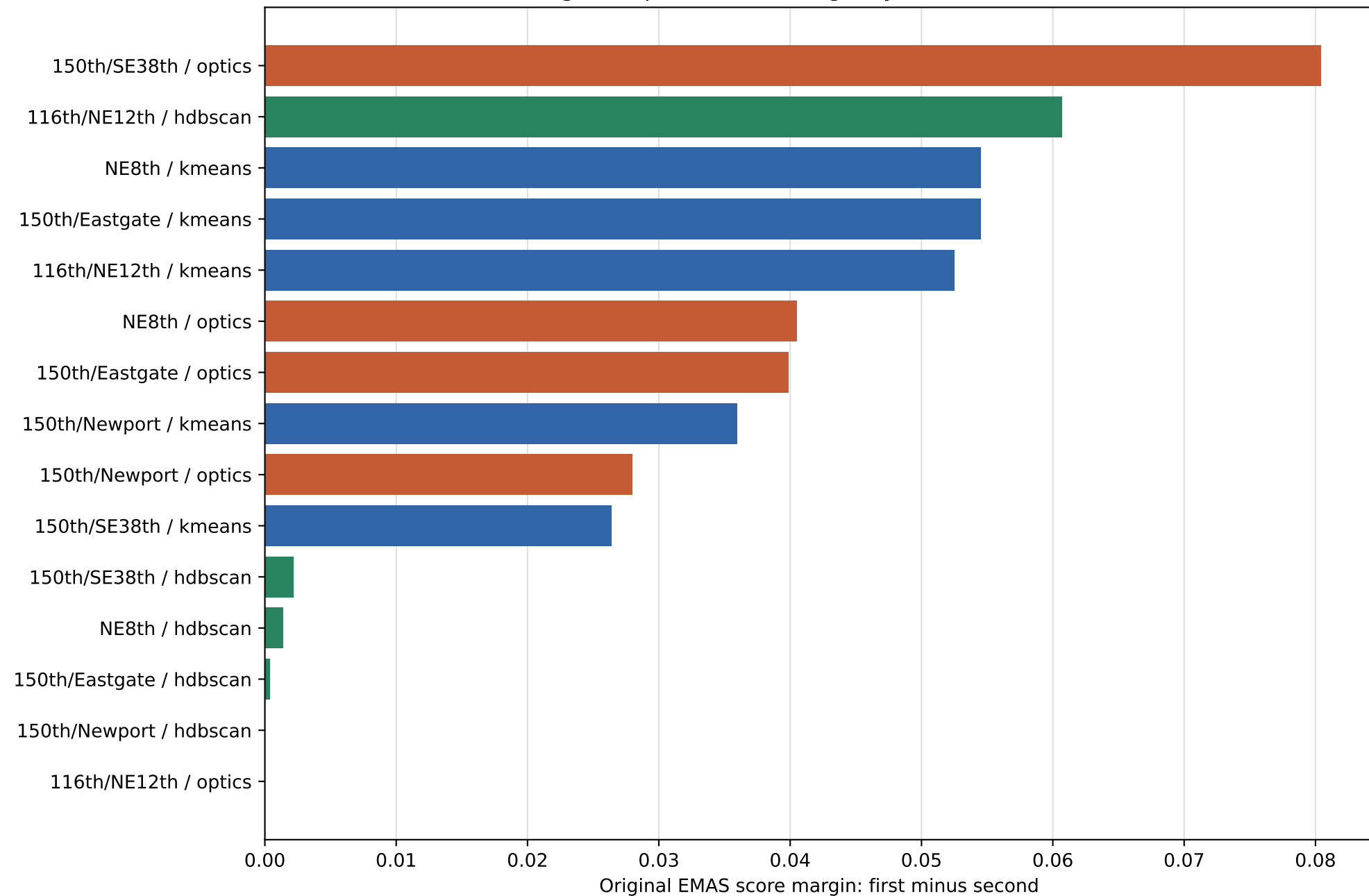
Original top-candidate margin by scene and method
