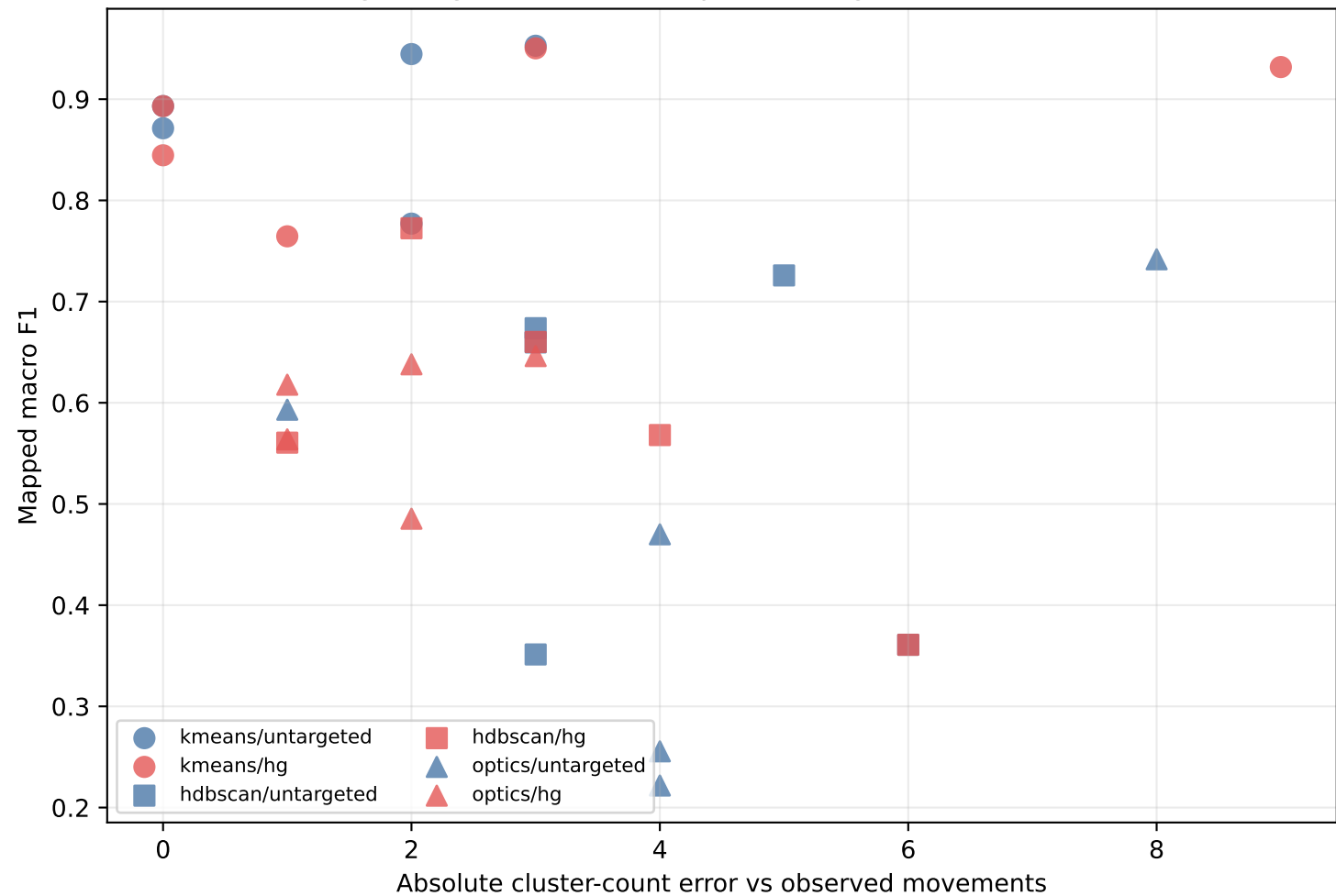
Target alignment and independent agreement trade-off
