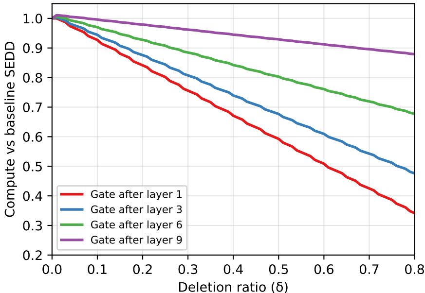
MrSEDD compute savings by gate layer (seq_len=128)
