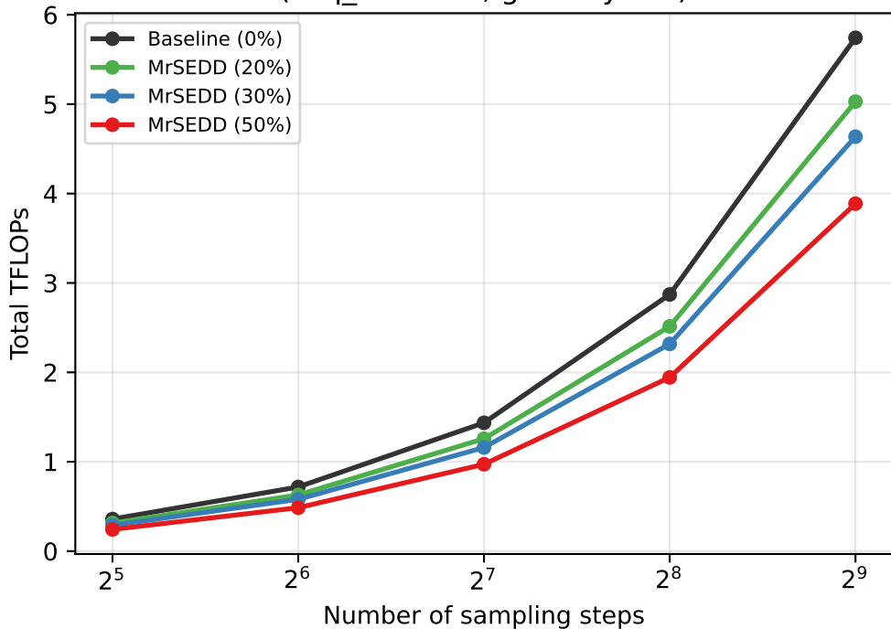
Total sampling compute: SEDD vs MrSEDD (seq_len=128, gate layer 3)
