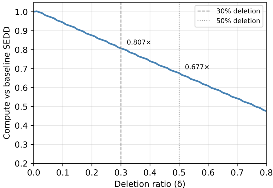
MrSEDD per-step compute savings (gate at layer 3, seq_len=128)
