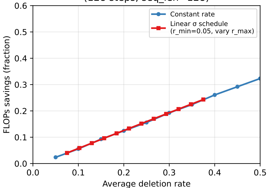
Sampling FLOPs savings: constant vs \sigma -schedule (128 steps, seq_len=128)
