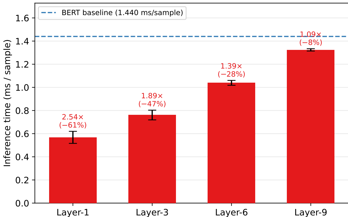
Inference runtime vs. gate layer placement (MrBERT-30%, SNLI, A100, hard deletion)
