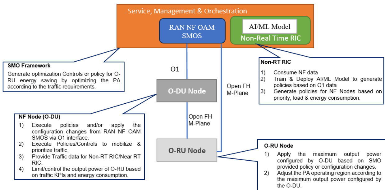
Figure 4.21.3.5-1: PA power optimization-based energy saving - Non-RT RIC and O1 based solution
