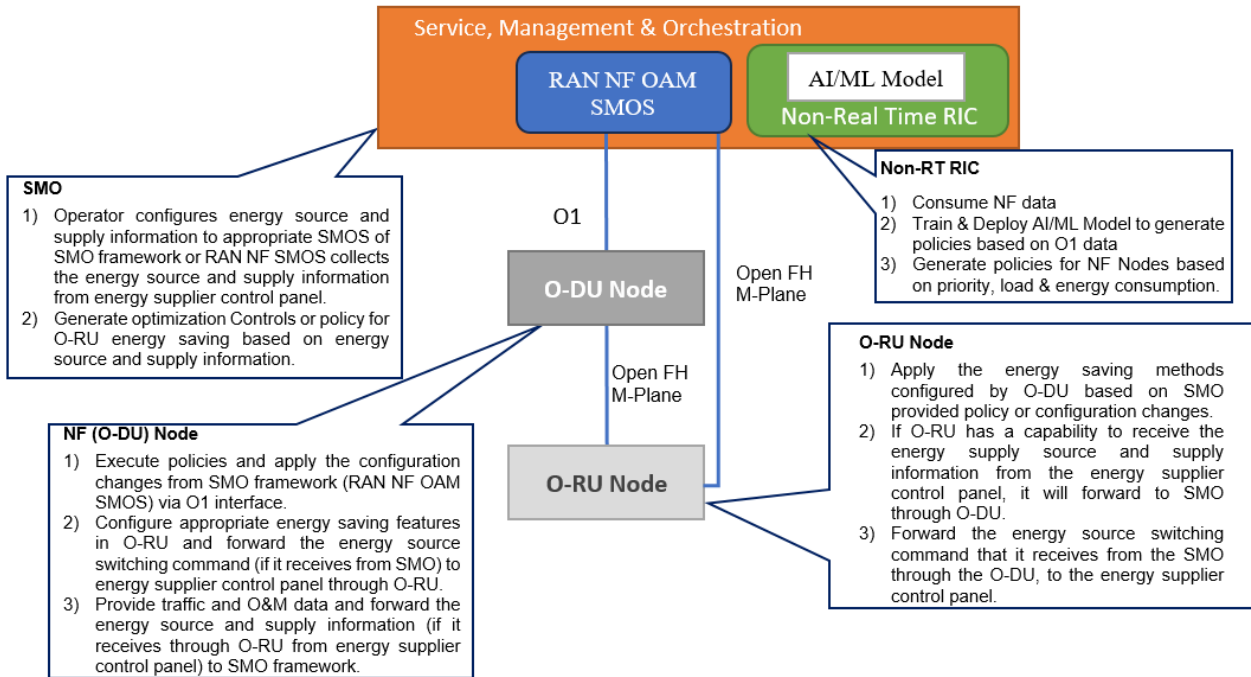
Figure 4.21.3.4-1: External power source coordination-based energy saving - Non-RT RIC and O1 based solution
