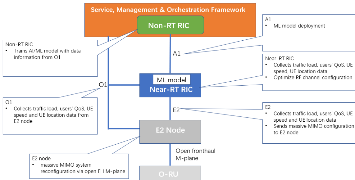
Figure 4.21.3.2-2: RF channel switch off/on ES sub-use case: Near-real-time implementation
