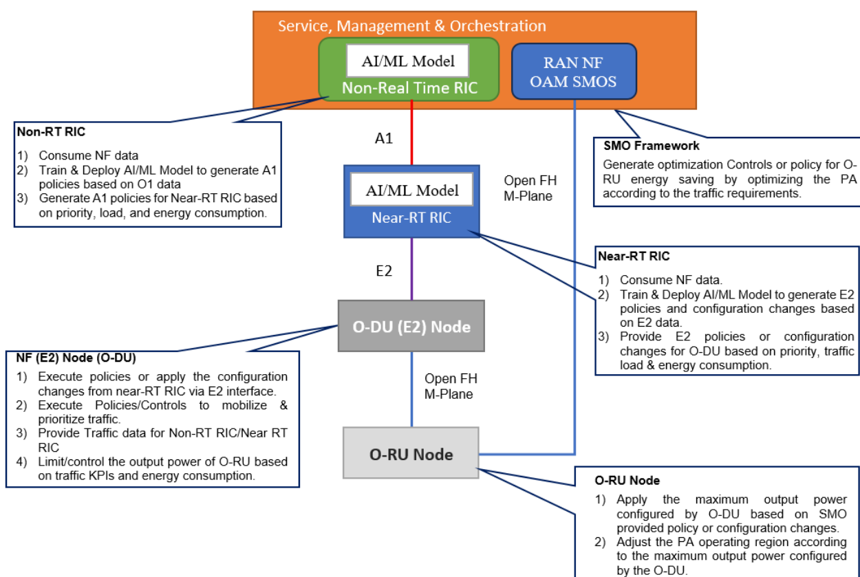
Figure 4.21.3.5-2: PA power optimization-based energy saving - Near-RT RIC and E2 based solution
