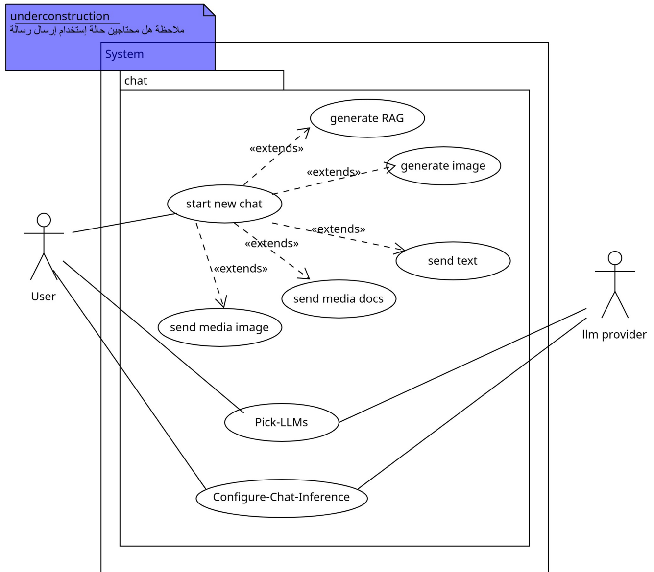
شكل 1: Chat-Use-Case-Diagram
