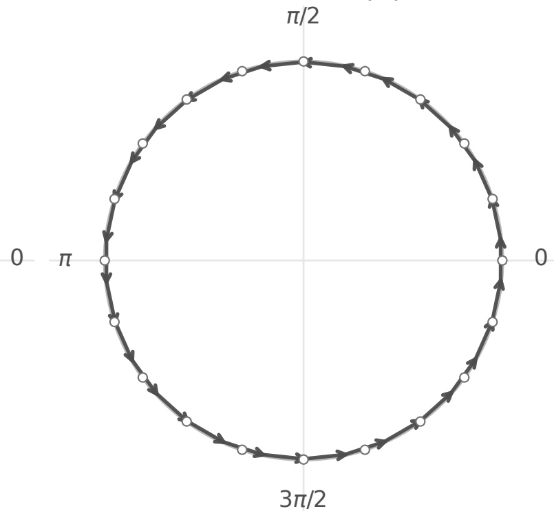
No fixed point: |a| < 1
