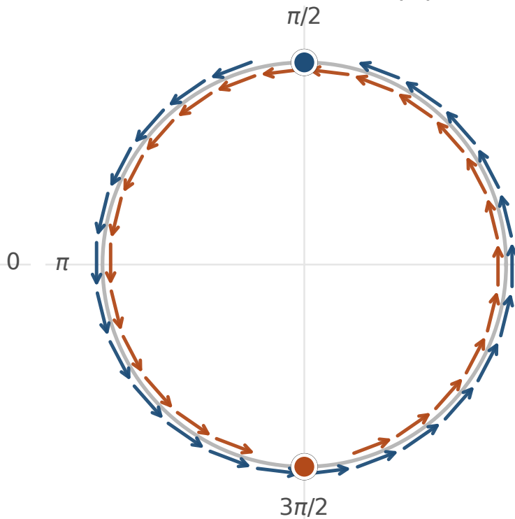
Critical fixed point: |a| = 1
