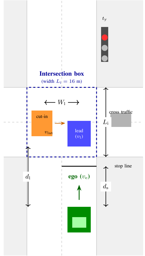
Fig. 1. Scene geometry for a northbound ego vehicle. The ego approaches a stop line at distance d_s ahead of the intersection box of width L_i ; a lead vehicle travelling at v_1 is inside the box in the ego lane; an adjacent vehicle with an active turn signal is preparing to cut into the ego lane from a lateral distance W_1 .
