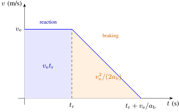
Fig. 2. Velocity-time profile under maximum braking (Theorem 11). The rectangle of height v_e and width t_r contributes the reaction distance v_e t_r ; the triangle of height v_e and base v_e/a_b contributes the braking distance v_e^2/(2a_b) . The total area is d_{\text{req}}(v_e) .
