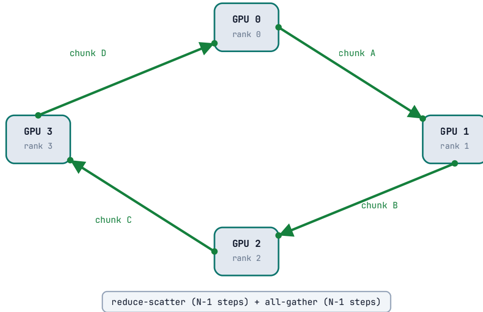
NCCL ring all-reduce (N = 4 GPUs)
