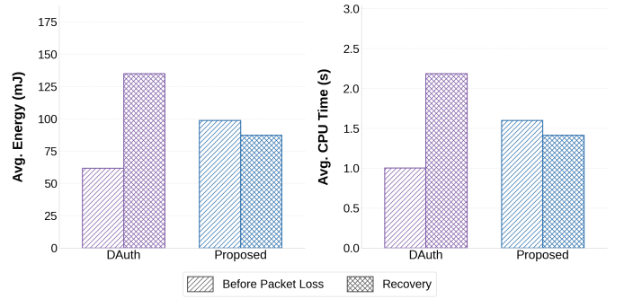
Fig. 8. Per-device desynchronisation recovery cost: (a) energy and (b) CPU time for a normal round vs. a recovery round, averaged over 20 devices in a 100-node network.
