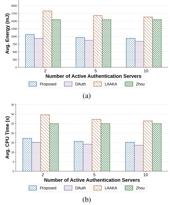
Fig. 6. Average authentication overhead vs. number of active authentication servers (20 devices): (a) energy and (b) CPU time.
