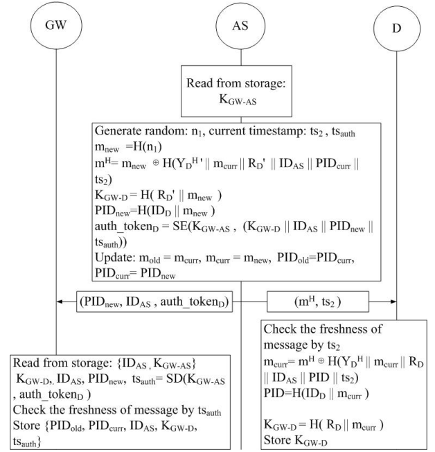
Fig. 3. Node Session Key Exchange Phase
