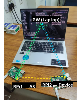
Fig. 9. Hardware testbed showing two Raspberry Pi 4B boards serving as the authentication server (left) and device (right), connected to a Windows laptop acting as the gateway.
