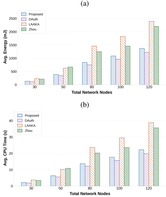
Fig. 7. Network scalability: (a) Avg. energy and (b) Avg. CPU time vs. network size N .
