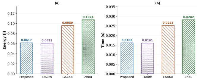
Fig. 10. Avg. Energy (a) and CPU time (b)
