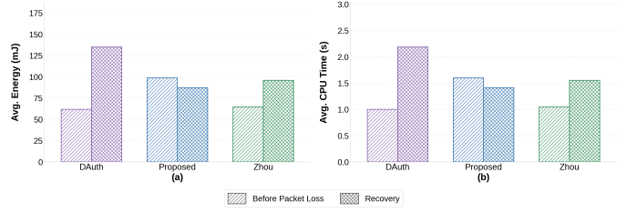
Fig. 8. Per-device desynchronisation recovery cost: (a) energy and (b) CPU time for a normal round vs. a recovery round, averaged over 20 devices in a 100-node network (5 seeds).
