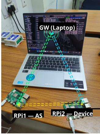
Fig. 9. Hardware testbed showing two Raspberry Pi 4B boards serving as the authentication server (left) and device (right), connected to a Windows laptop acting as the gateway.
