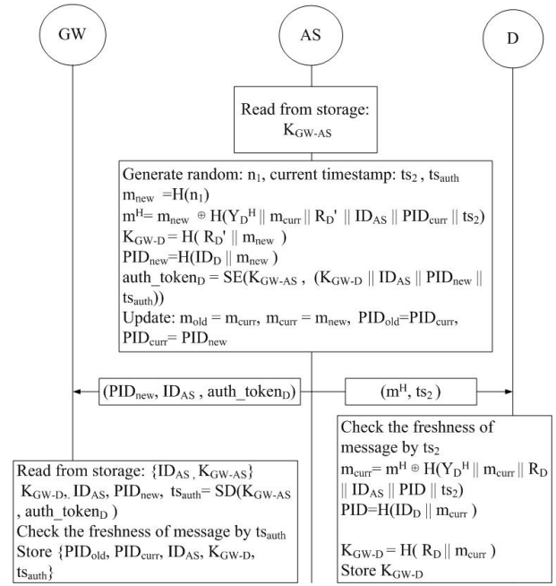
Fig. 3. Session Key Exchange Phase via open channel.
