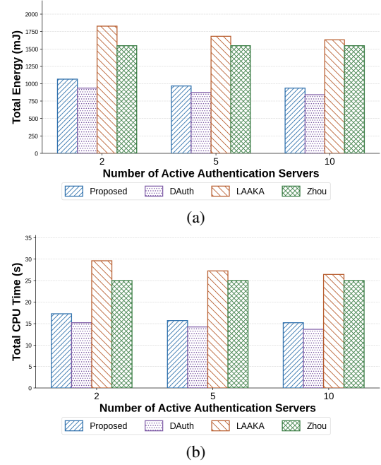
Fig. 6. Total authentication cost vs. number of authentication servers (20 devices): (a) energy and (b) CPU time.
