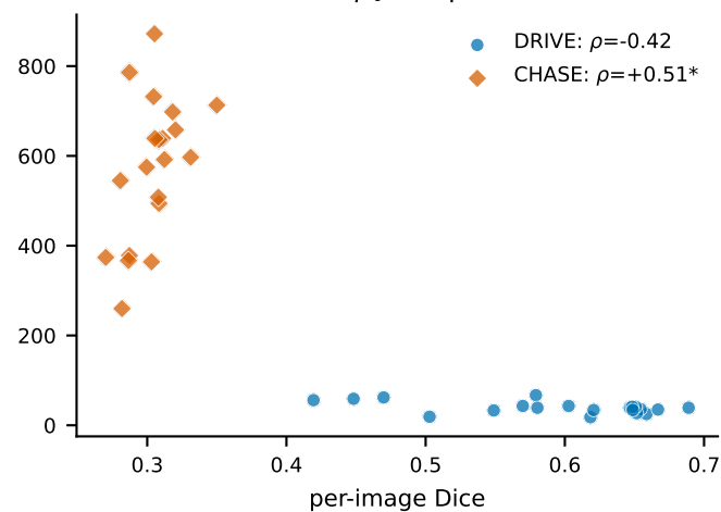
certified \beta_0 components
