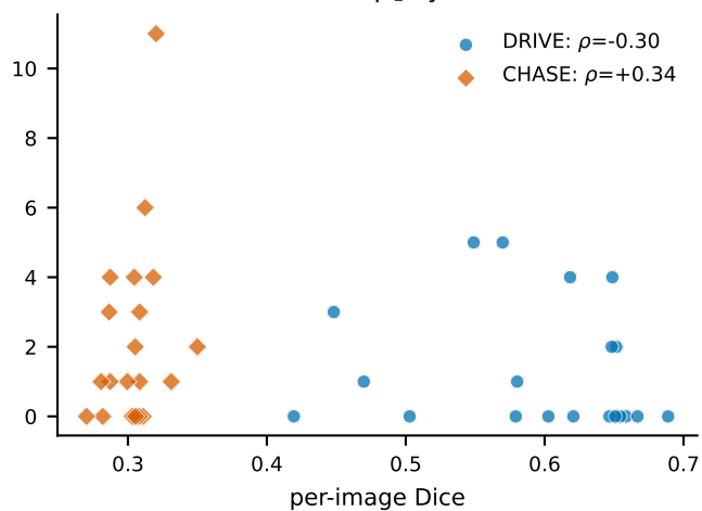
certified \beta_1 cycles
