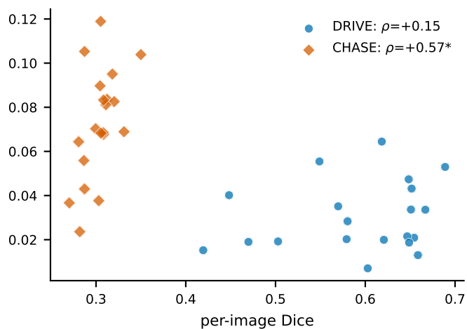
certified \beta_1 cycles
